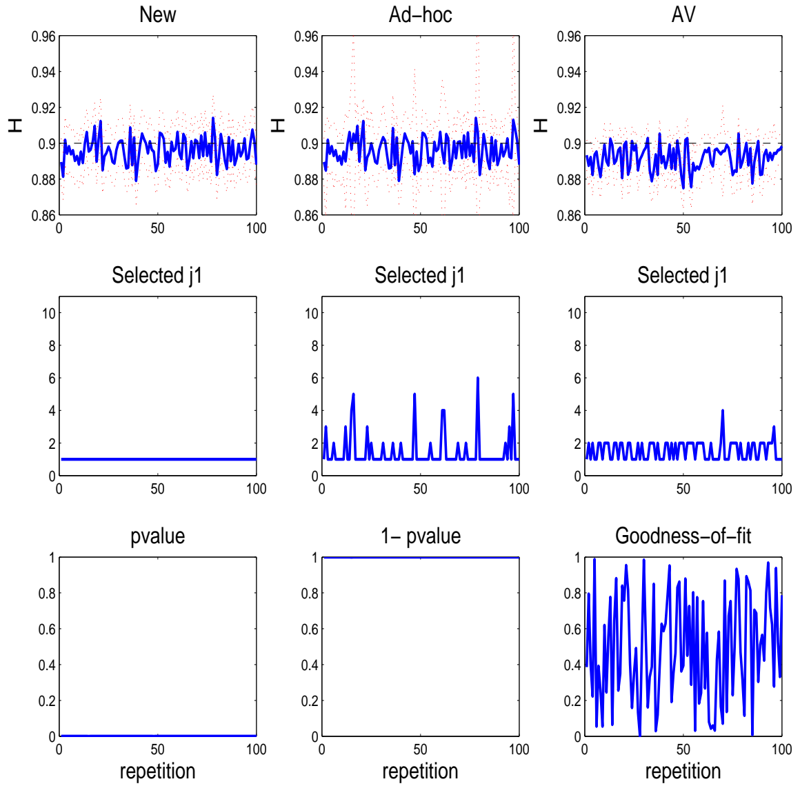
Figure 4: FGN ( H = 0.9 )
